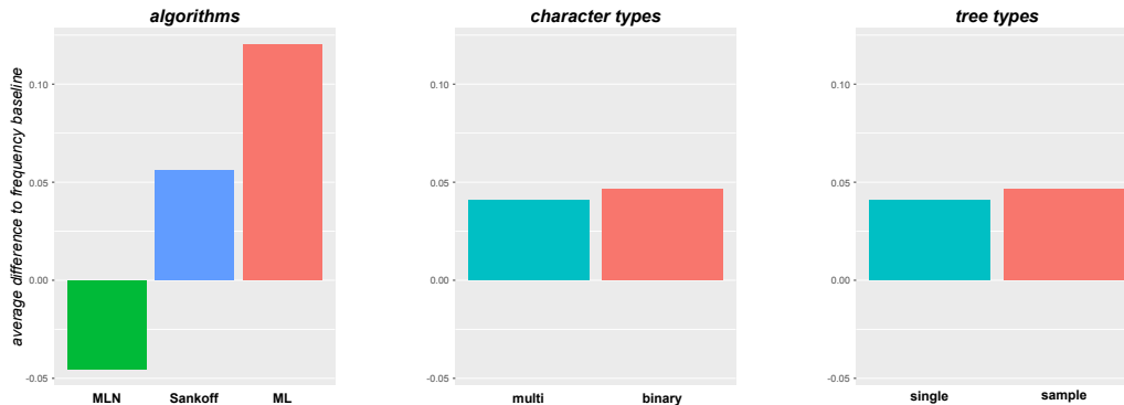
Figure 6 Average differences in F-score to frequency baseline
